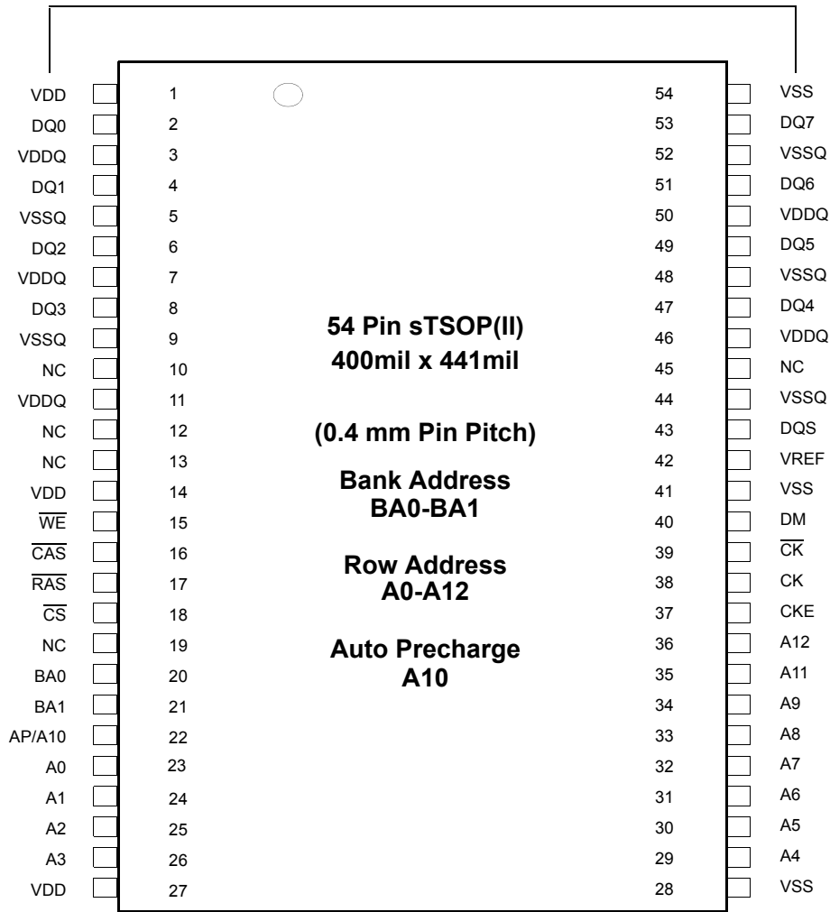
512Mb sTSOP(II)-400 Package Pinout
