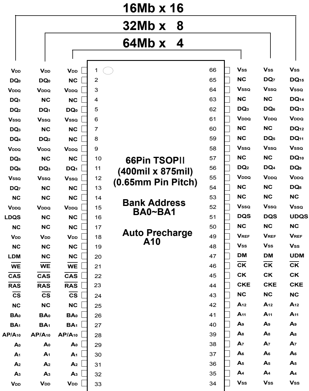
256Mb TSOP-II Package Pinout
