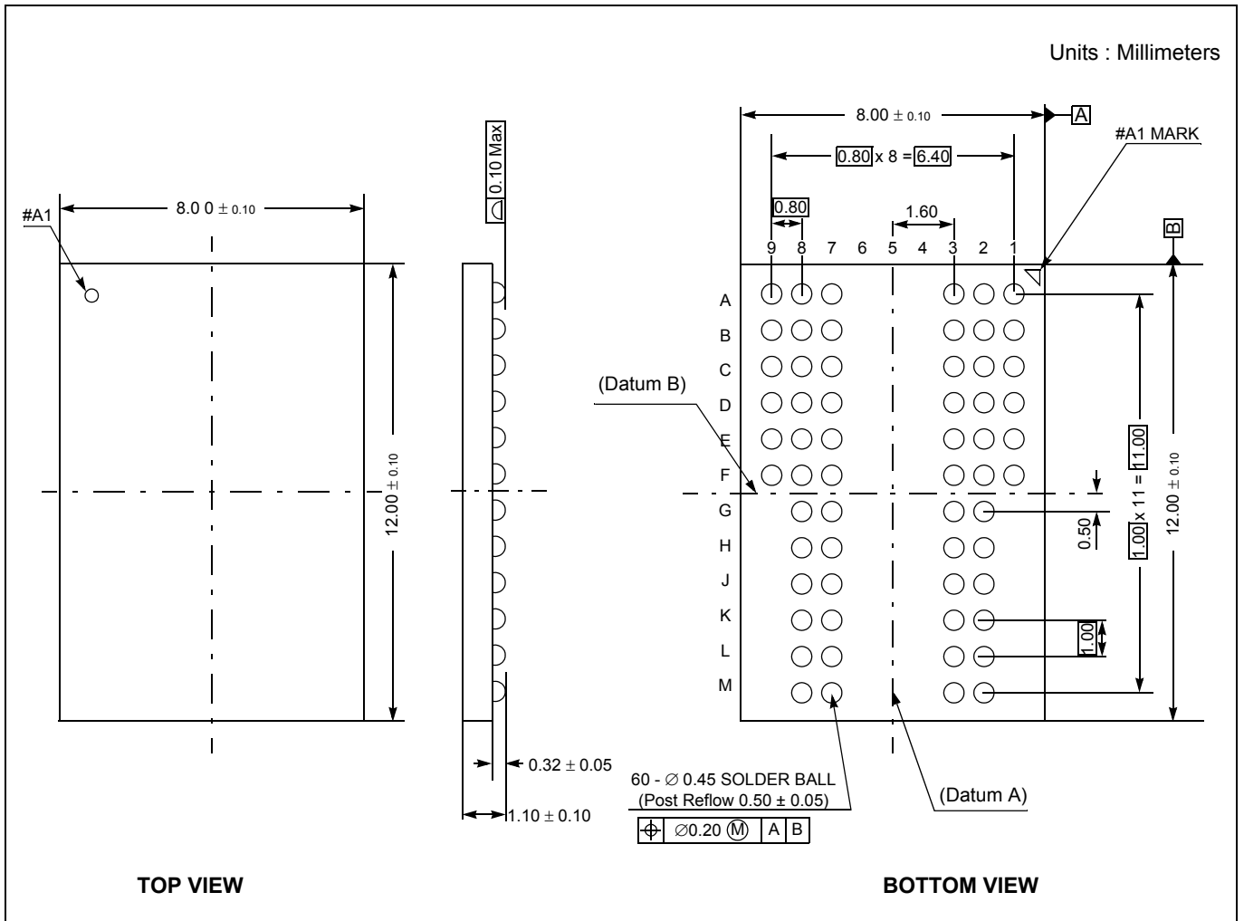
60Ball FBGA 64Mb Package Dimension
