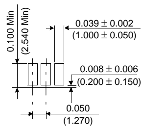
Detail C
