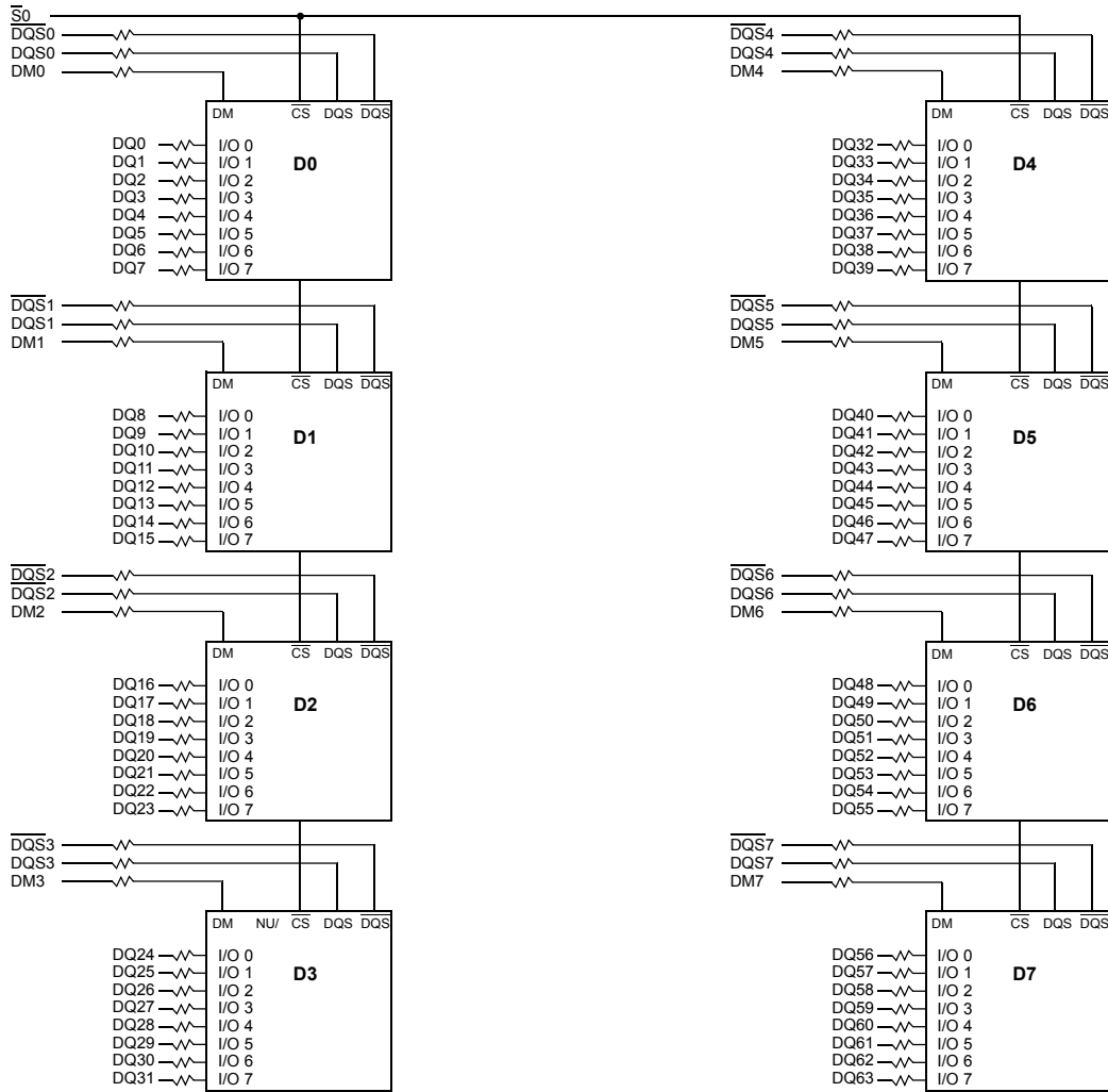
Functional Block Diagram: 512MB, 64Mx64 Module (Populated as 1 rank of x8 DDR2 SDRAMs) M378T6553BG(Z)3 / M378T6553BG(Z)0
