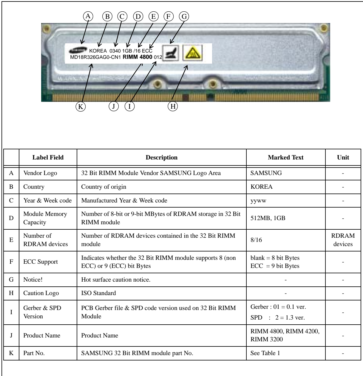
Figure 5 : 32 Bit RIMM Module Marking Example
