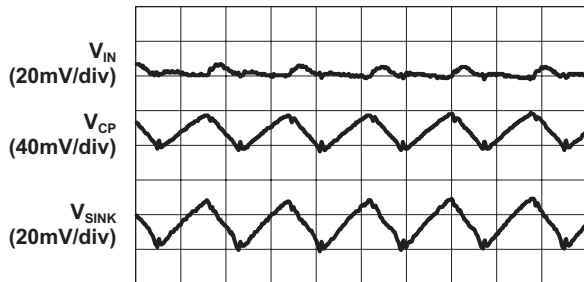
Load Characteristics ( V_{IN} = 3.7V ; 1.5X Mode; 20mA/ch Load)
