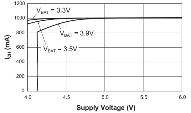
Fast Charge Current vs. Supply Voltage (ADPSET = 8.06k \Omega )
