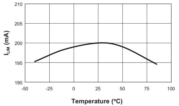
I_{LIM} vs. Temperature ( V_{IN} = 4V ; V_{OUT} = 3.85V ; ENLB = 0V ; R_{SET} = 249k\Omega )
