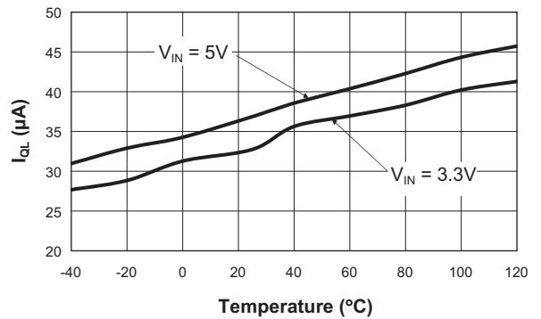
Quiescent Current I_{QL} vs. Temperature ( ENLB = 0V ; ENUB = V_{CC} ; V_{OUT} = Open )
