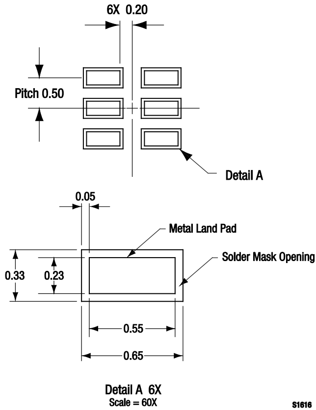
Figure 8. AS211-334 PCB Layout Footprint (Top View)
