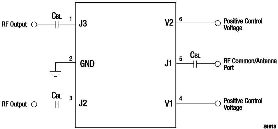
Figure 7. AS211-334 Evaluation Board Schematic
