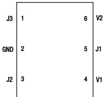
Figure 2. AS211-334 Pinout – 6-Pin DFN (Top View)
