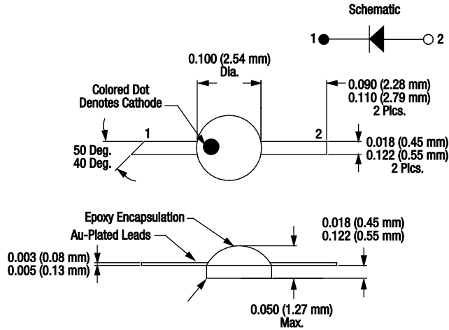
Figure 13. -250 Package Dimensions
