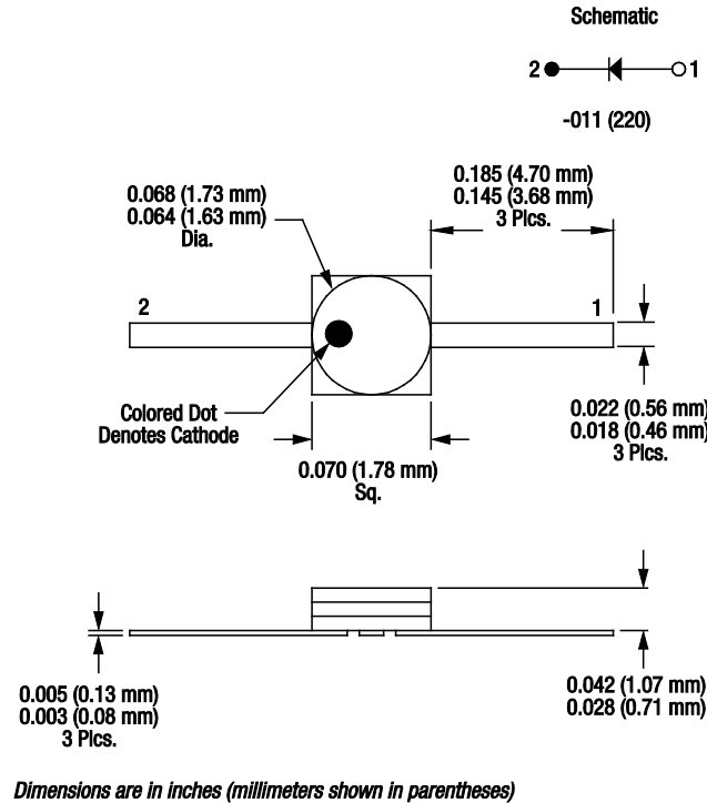
Figure 12. -220 Package Dimensions
