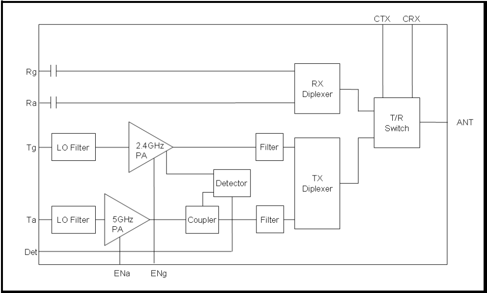
Figure 1: SE5503A Functional Block Diagram
