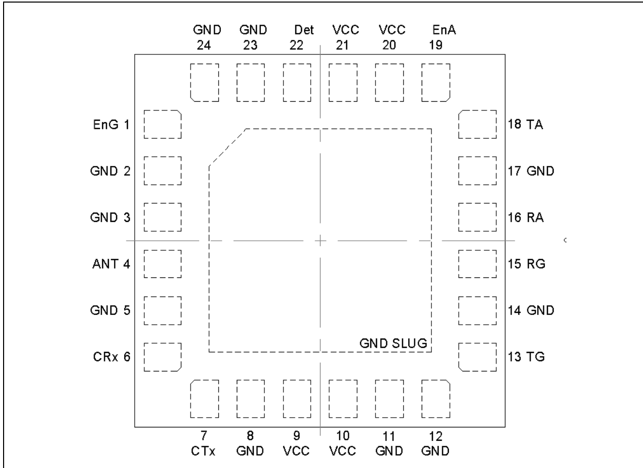
Figure 2: SE5503A Pin Out (Top View Through Package)
