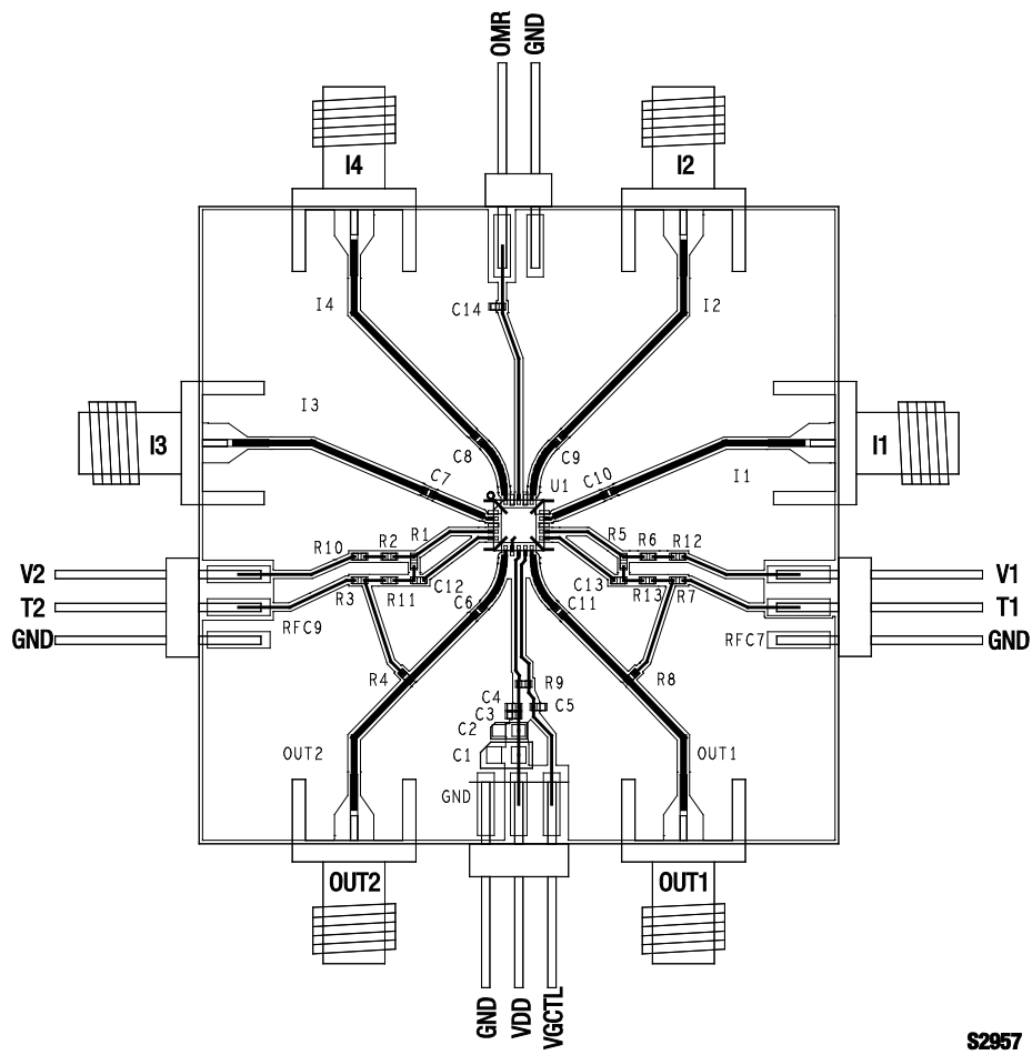
Figure 12. SKY13419-365LF Evaluation Board Assembly Diagram
