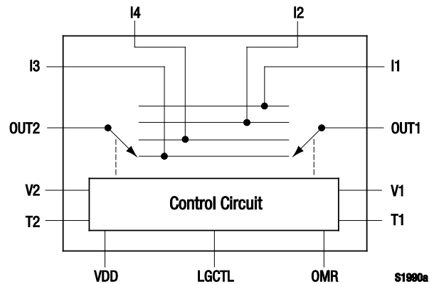
Figure 1. SKY13419-365LF Block Diagram
