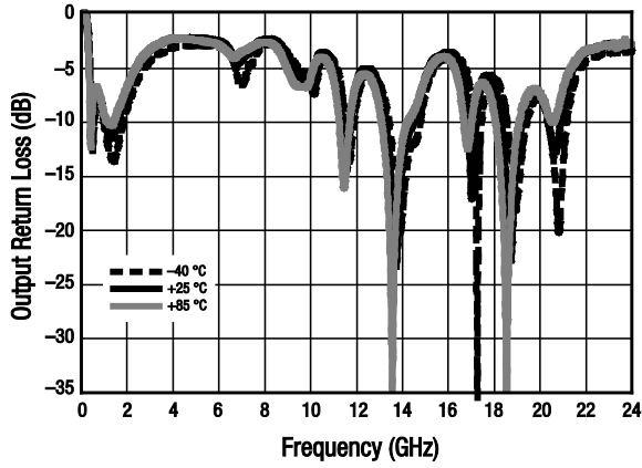
Figure 11. Small Signal Output Return Loss (S22) vs Frequency and Temperature, Wide Band
