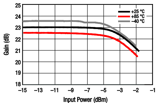
Figure 20. Gain vs Input Power Over Temperature @ 500 MHz
