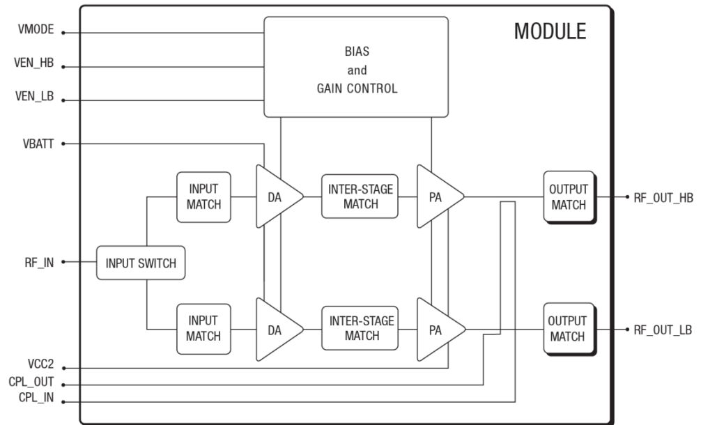
Figure 1. SKY77742 Functional Block Diagram
