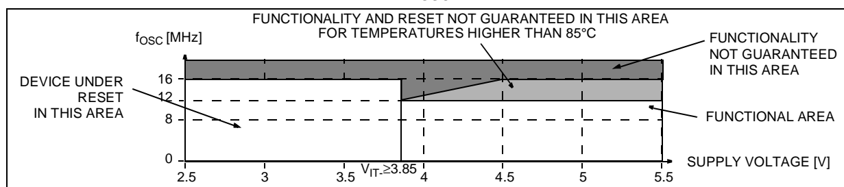
Figure 58. Medium LVD Threshold Versus V_{DD} and f_{OSC} for FLASH devices 2)
