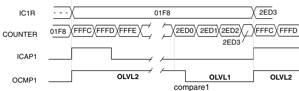
Figure 53. One Pulse Mode Timing Example
