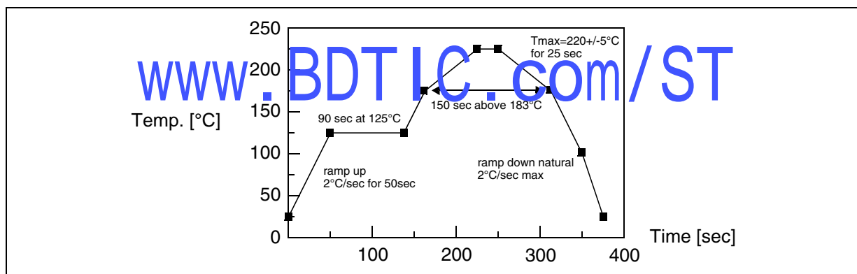
Figure 47. Recommended Reflow Oven Profile (MID JEDEC)
