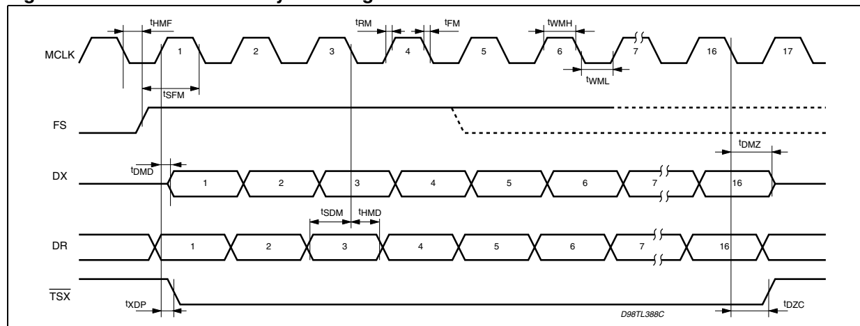
Figure 10. MCU mode frame sync. timing
