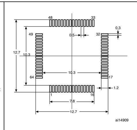
Figure 59. Recommended footprint (1)(2)
