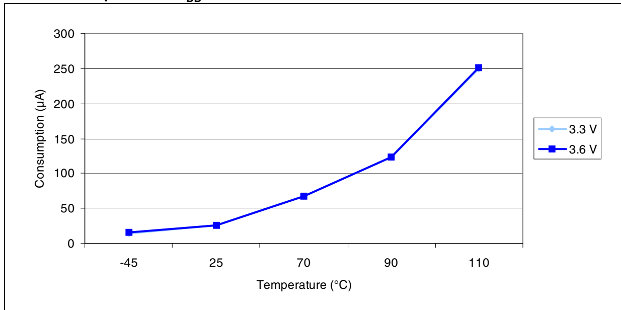
Figure 15. Typical current consumption in Stop mode with regulator in Run mode versus temperature at V_{DD} = 3.3\text{ V} and 3.6\text{ V}
