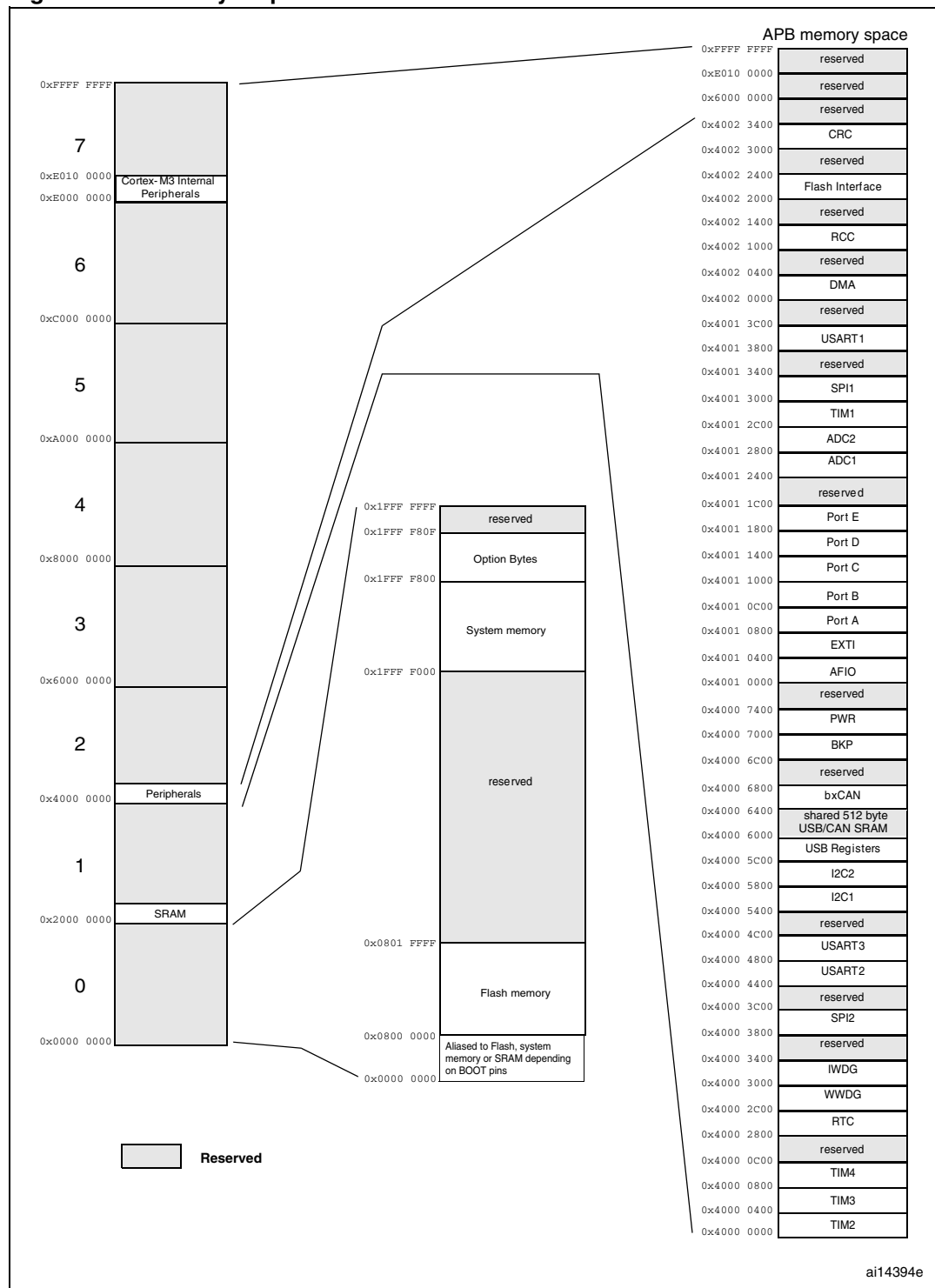
Figure 8. Memory map
