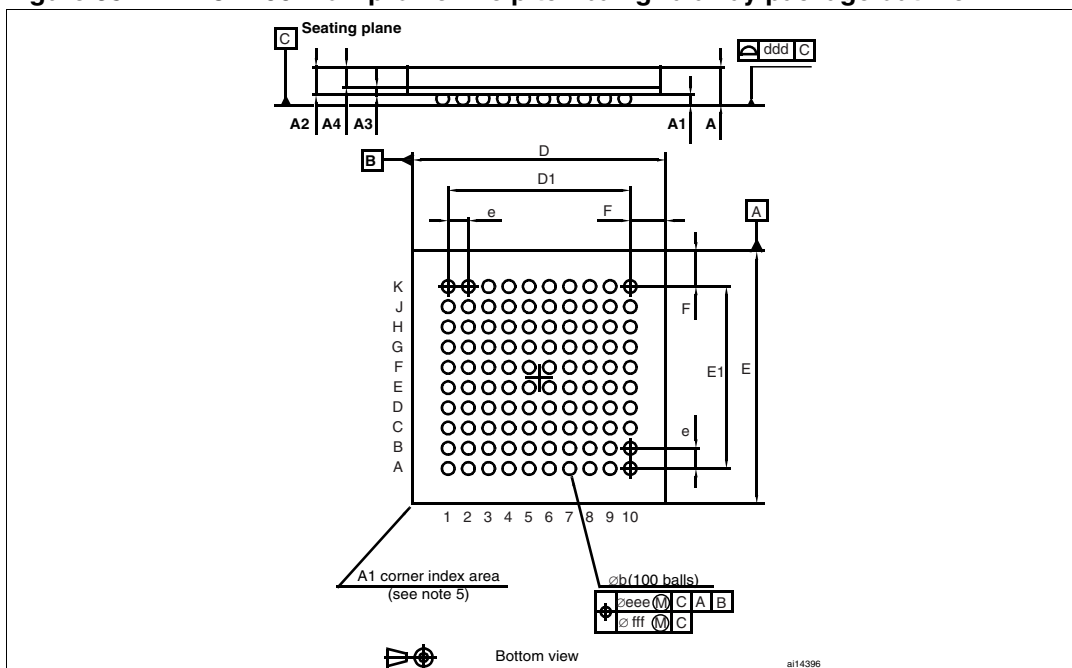
Figure 35. LFBGA100 - low profile fine pitch ball grid array package outline
