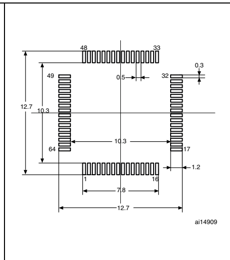
Figure 40. Recommended footprint (1)(2)
