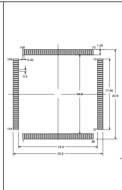
Figure 81. Recommended footprint (1)(2)
