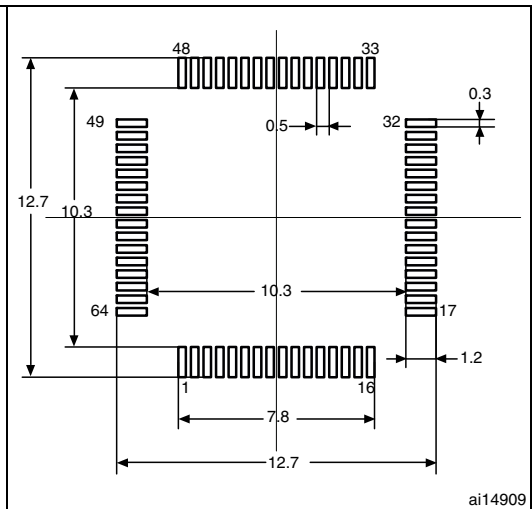
Figure 76. Recommended footprint (1)(2)
