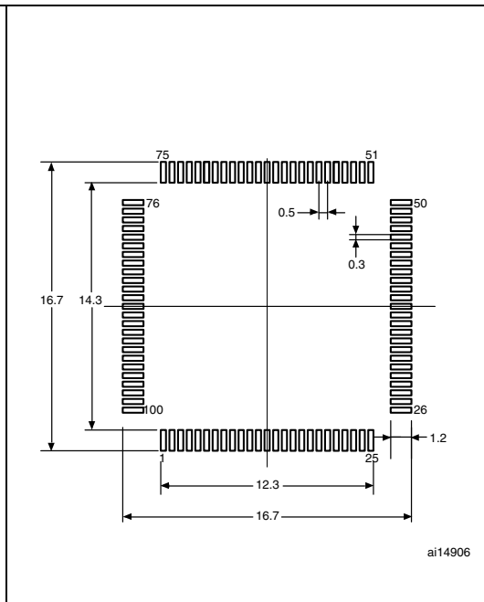
Figure 77. Recommended footprint (1)(2)
