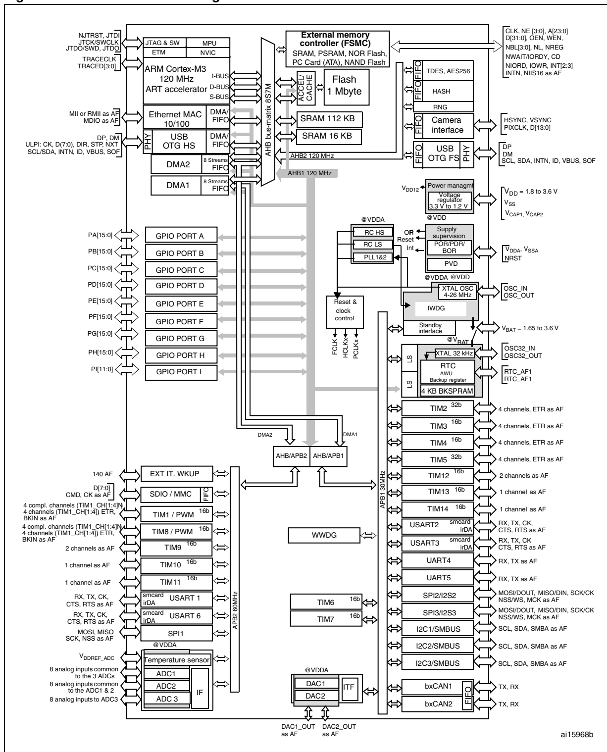
Figure 5. STM32F21x block diagram
