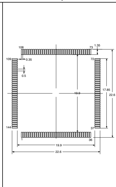
Figure 79. Recommended footprint (1)(2)
