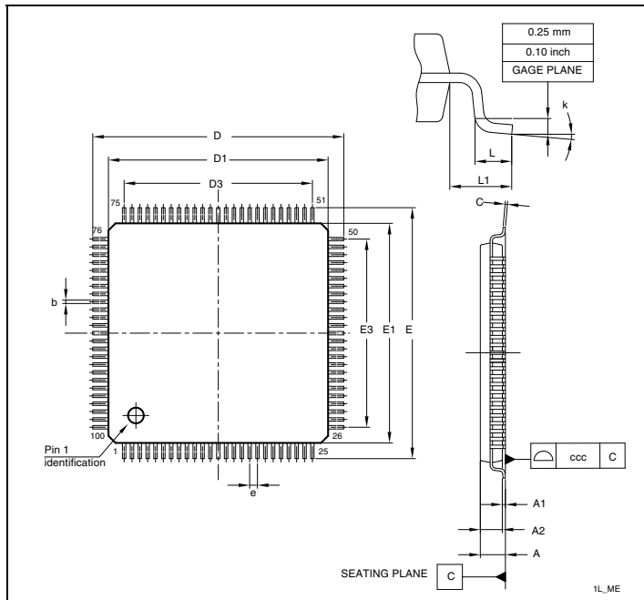
Figure 76. LQFP100, 14 x 14 mm 100-pin low-profile quad flat package outline (1)
