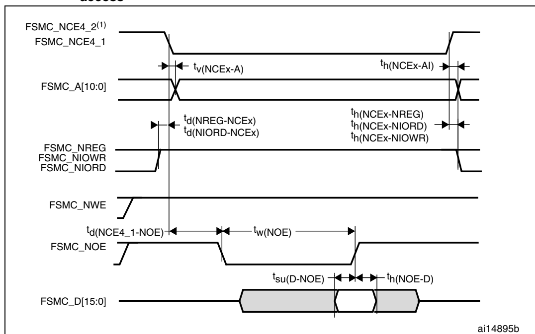
Figure 54. PC Card/CompactFlash controller waveforms for common memory read access
