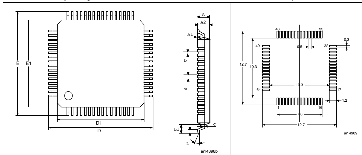
Figure 39. Recommended footprint (1)(2)
