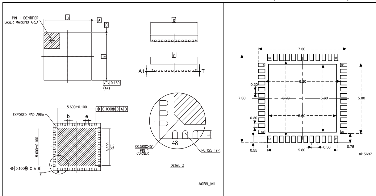
Figure 31. UFQFPN48 7 x 7 mm, 0.5 mm pitch, package outline (1)(2)(3)
