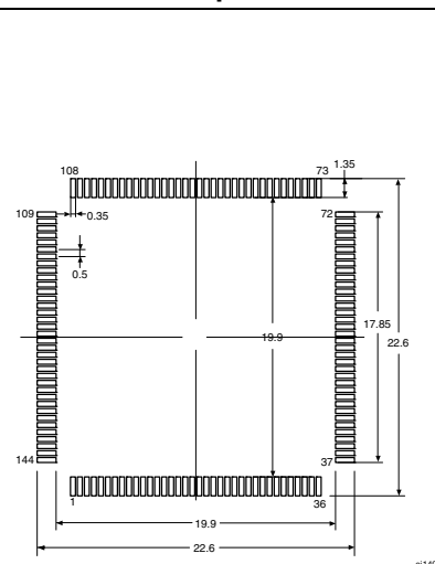
Figure 37. Recommended footprint
