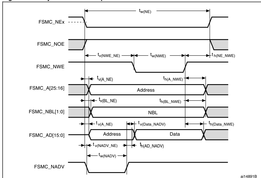
Figure 18. Asynchronous multiplexed PSRAM/NOR write waveforms
