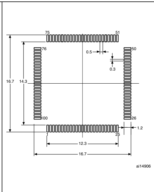
Figure 39. Recommended footprint
