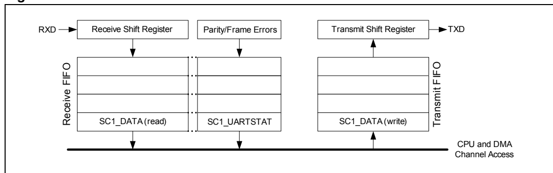
Figure 11. UART FIFOs
