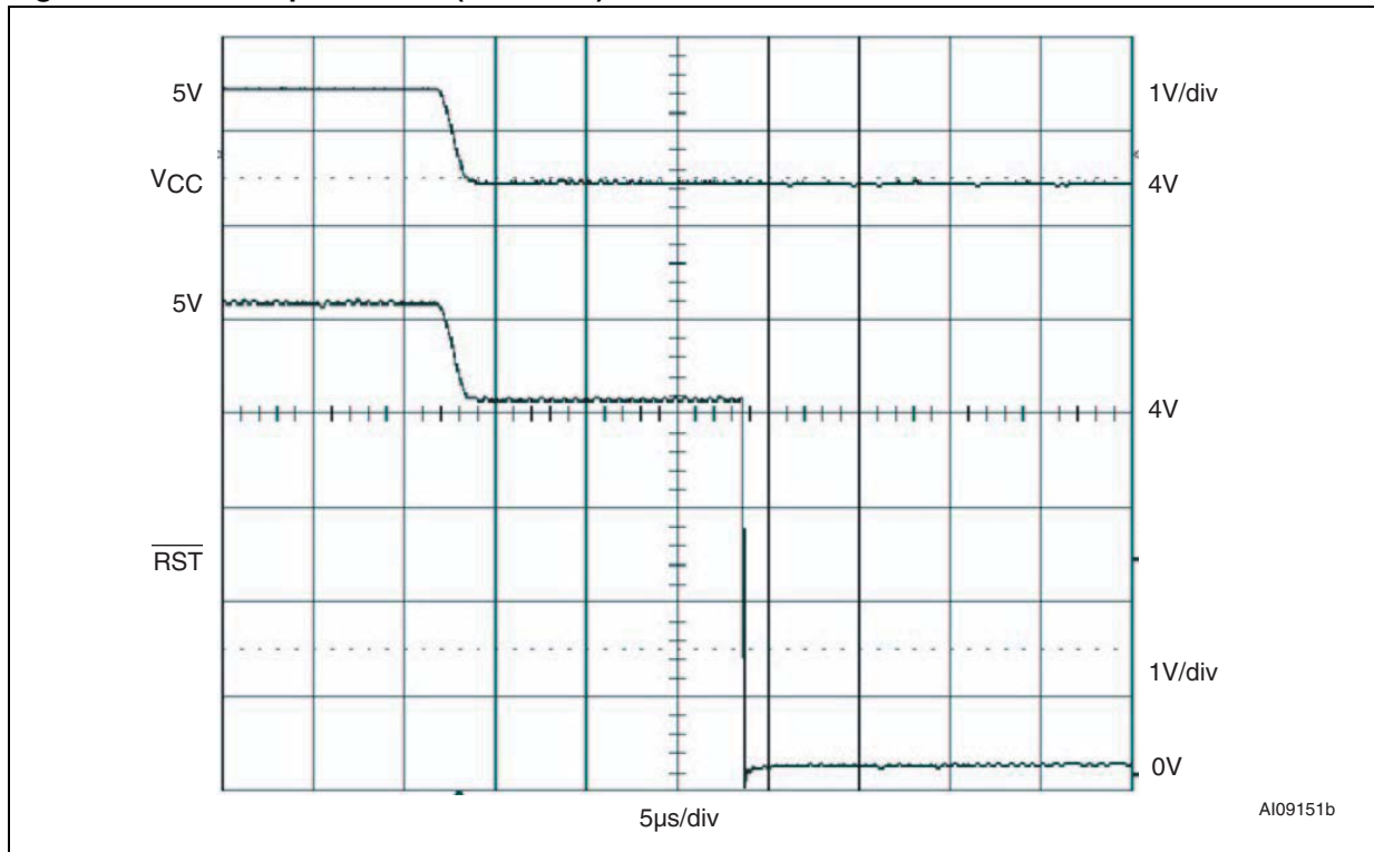
Figure 34. \overline{\text{RST}} response time (assertion)
