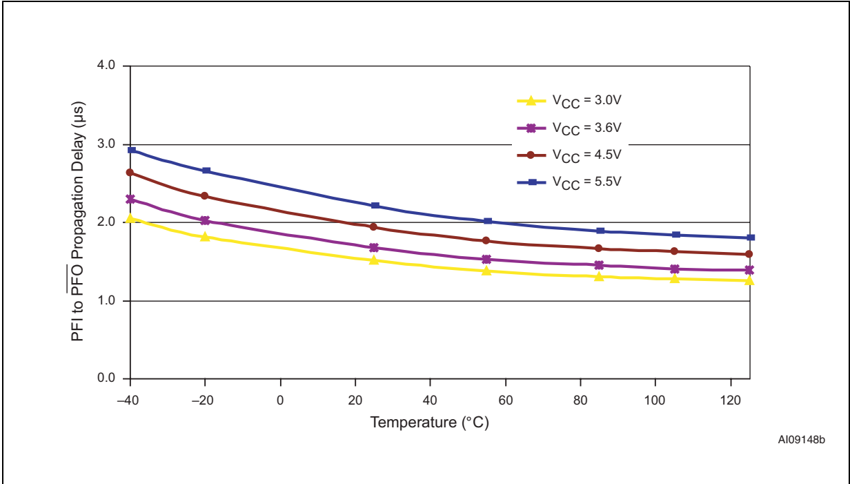
Figure 28. PFI to \overline{\text{PFO}} propagation delay vs. temperature
