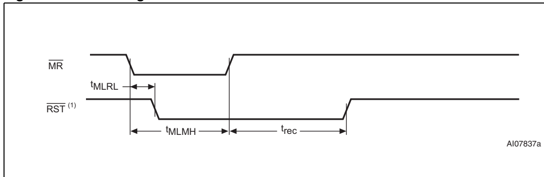
Figure 41. \overline{\text{MR}} timing waveform
