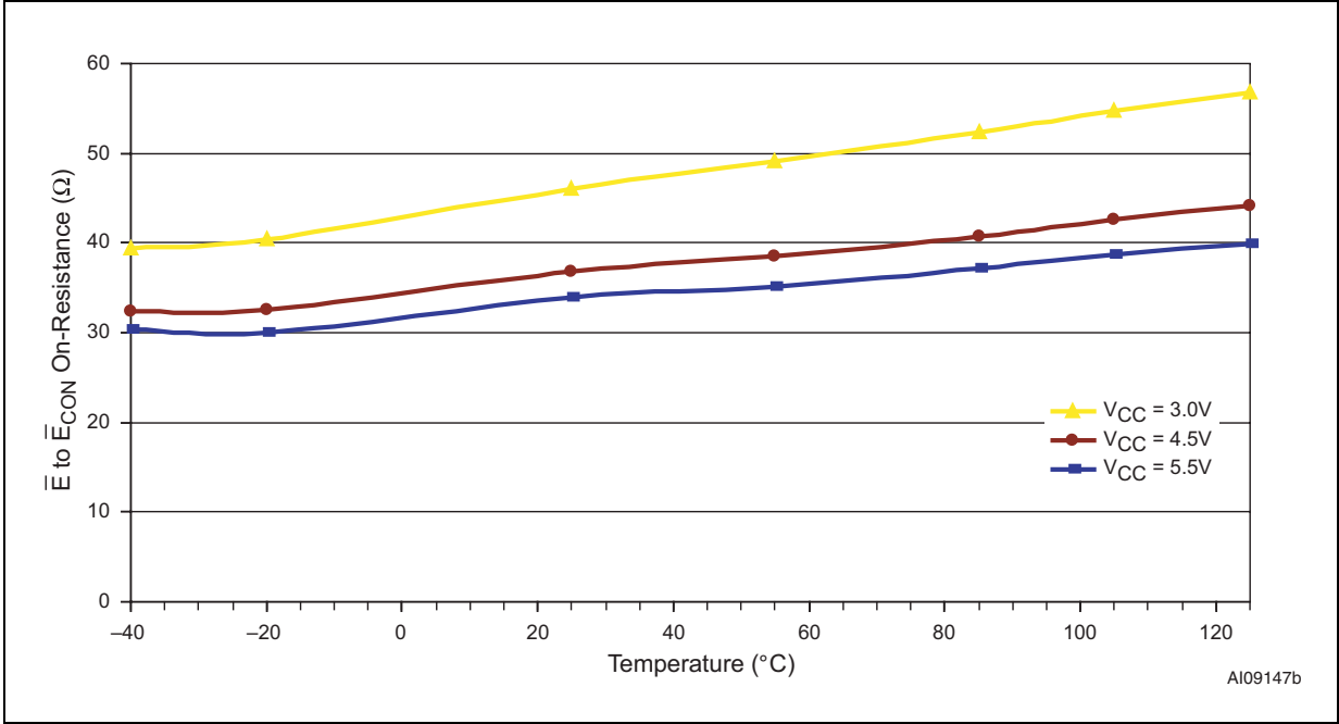
Figure 27. \bar{E} to \bar{E}_{CON} on-resistance vs. temperature
