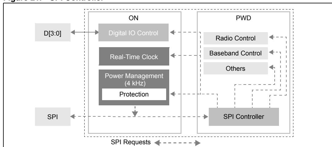
Figure 21. SPI Controller
