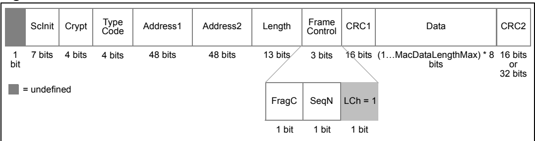
Figure 43. LCh field set to LCCh
