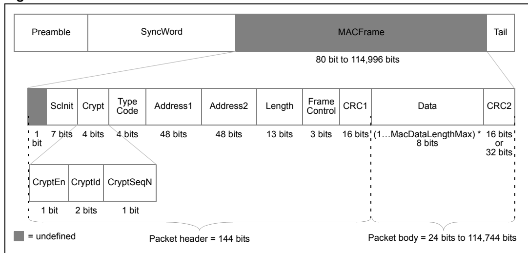
Figure 34. MACFrame field
