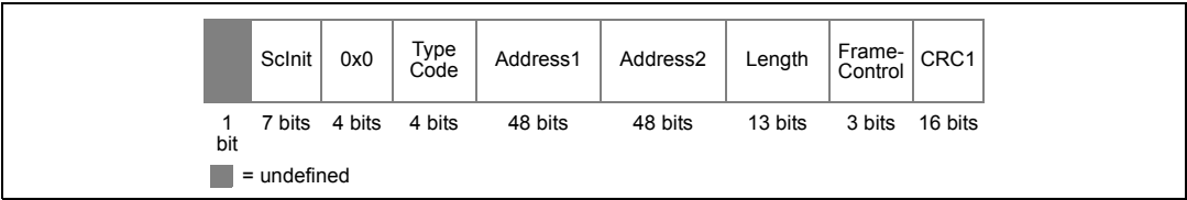
Figure 40. MACFrame format of Req2S packet
