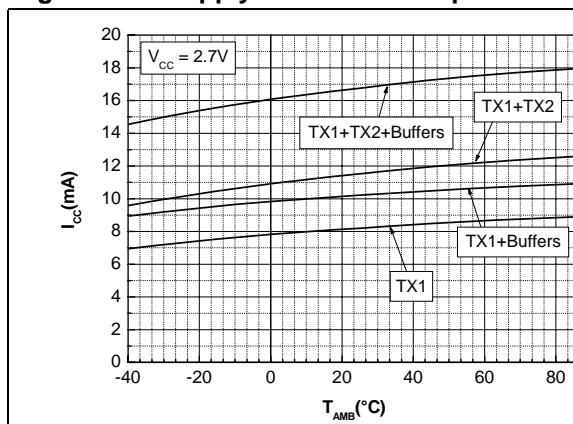
Figure 5. Supply current vs. temperature
