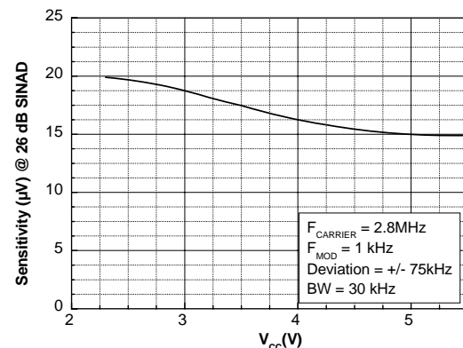
Figure 6. Sensitivity vs. supply voltage
