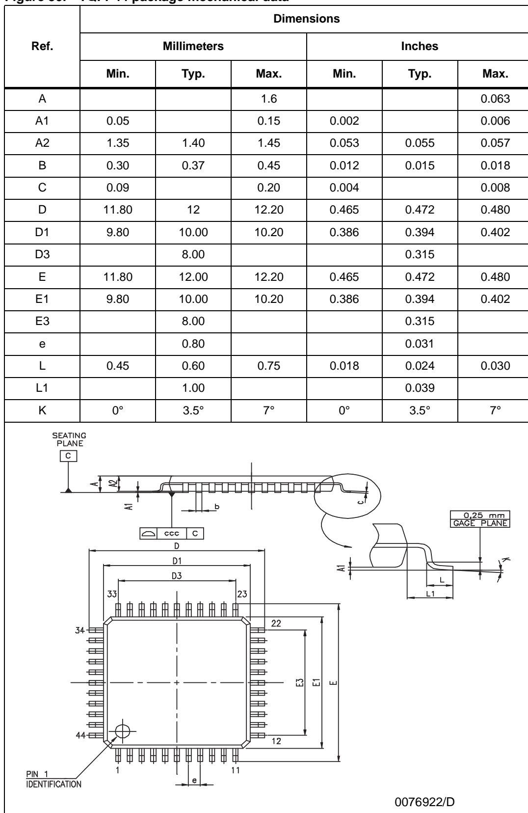
Figure 30. TQFP44 package mechanical data
