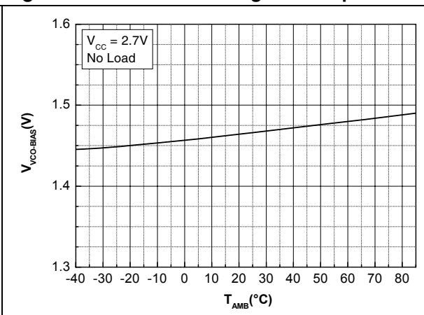
Figure 19. VCO-BIAS voltage vs. temperature
