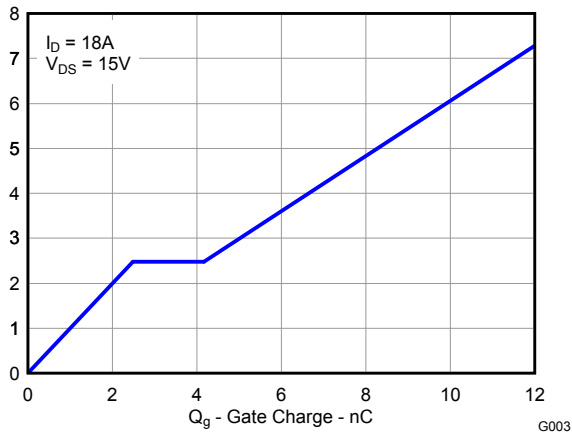
Figure 4. Gate Charge
