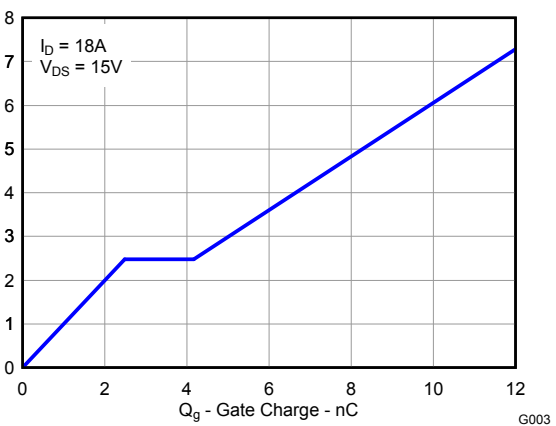
GATE CHARGE
