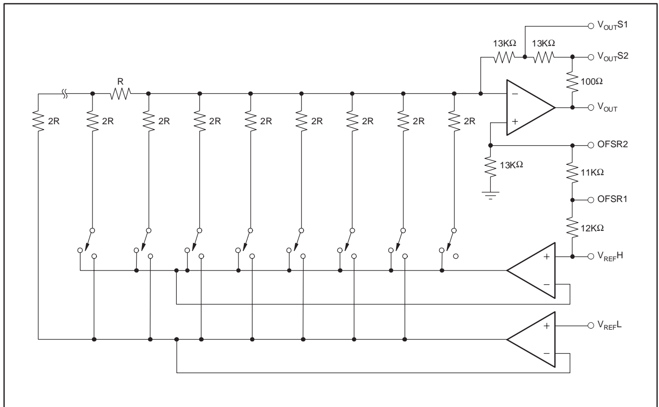
Figure 53. DAC7654 Architecture
