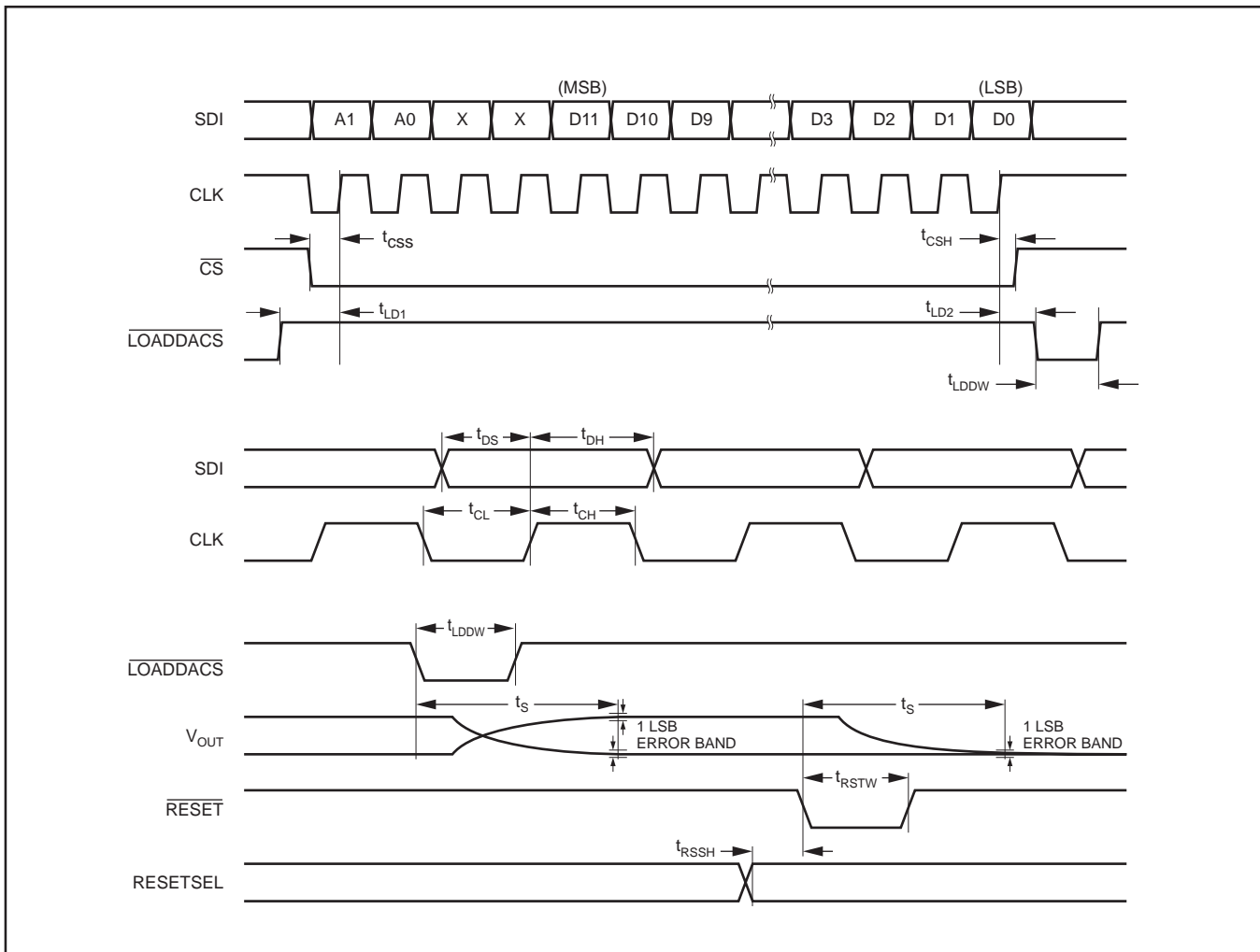
FIGURE 4. DAC7714 Timing.
