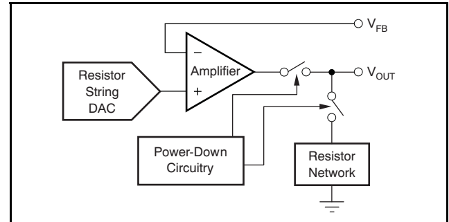
Figure 49. Output Stage During Power-Down
