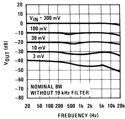
FIGURE 3. Output vs Frequency
