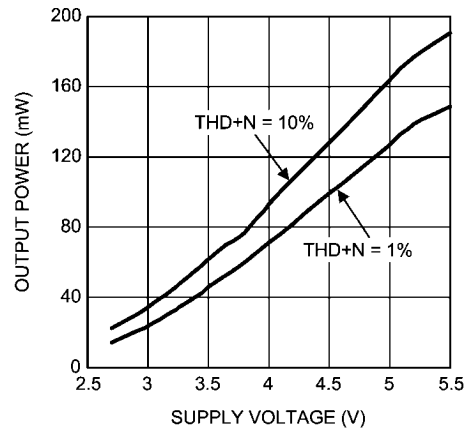
Output Power vs Supply Voltage R_L = 8\Omega , f = 1\text{kHz} Earpiece Bypass Mode
