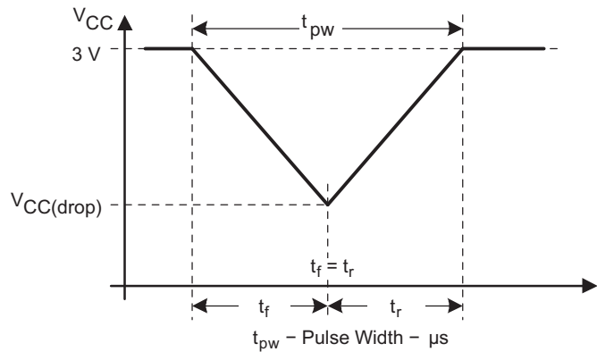
Figure 6. V CC(drop) Level With a Triangle Voltage Drop to Generate a POR/Brownout Signal
