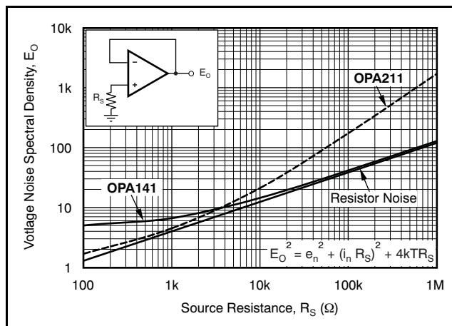
Figure 31. Noise Performance of the OPA141 and OPA2141 in Unity-Gain Buffer Configuration
