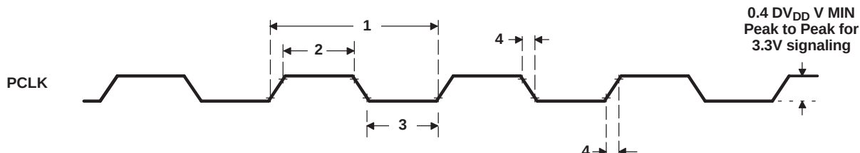
Figure 5-36. PCLK Timing
