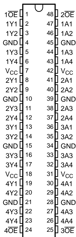
SN54ABT16244... WD PACKAGE SN74ABT16244A... DGG, DGV, OR DL PACKAGE (TOP VIEW)
