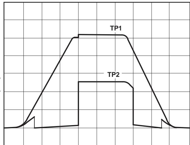
X-Axis = 0.2 ms/Division Figure 18. V CC vs Output Waveform 3
