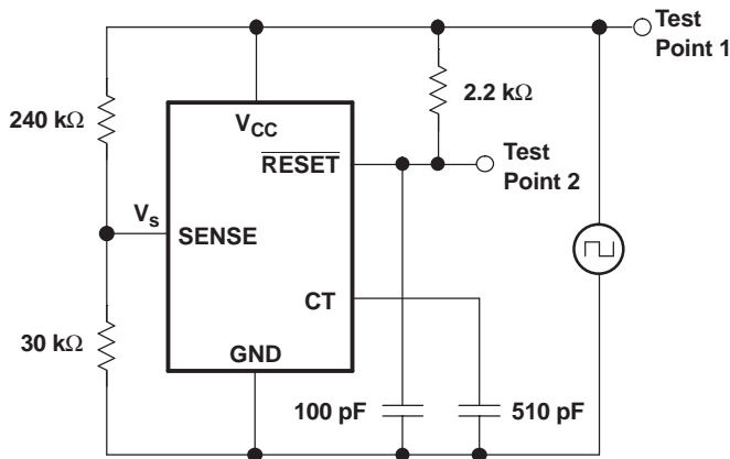
Figure 15. V CC vs Output Test Circuit 2
