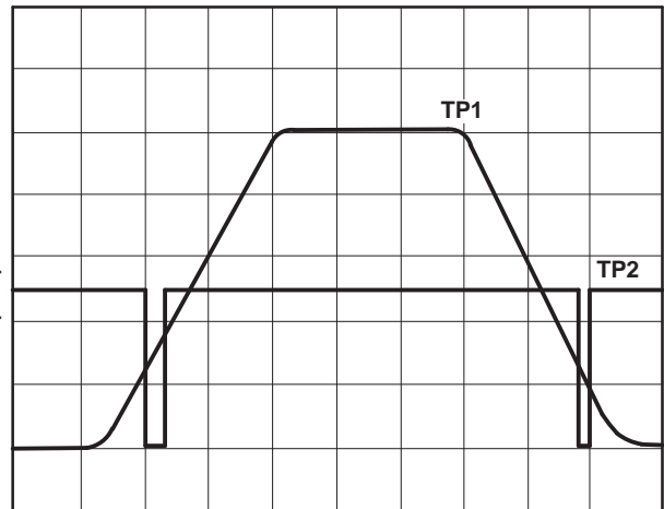
X-Axis = 0.2 ms/Division Figure 16. V CC vs Output Waveform 2
