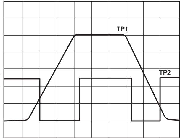
X-Axis = 0.2 ms/Division Figure 14. V CC vs Output Waveform 1
