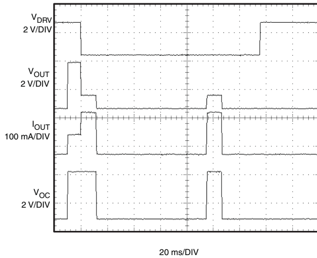
Figure 20. t_{RESTART} Response
