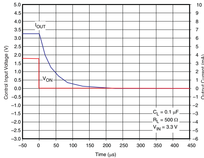
Figure 22. t_{ON} Response
