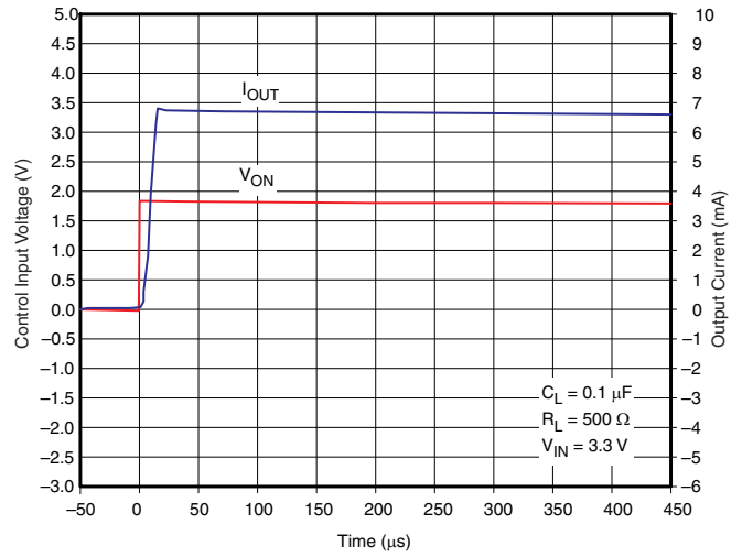
Figure 21. t_{ON} Response
