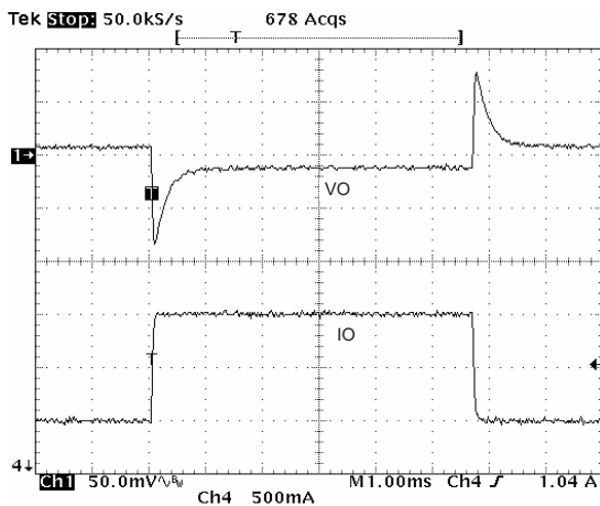
Figure 51. Load Transient
