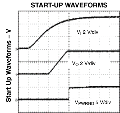
Time - 2 ms/div
