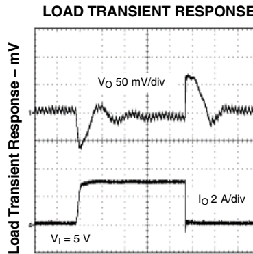
Time - 10 μs/div
