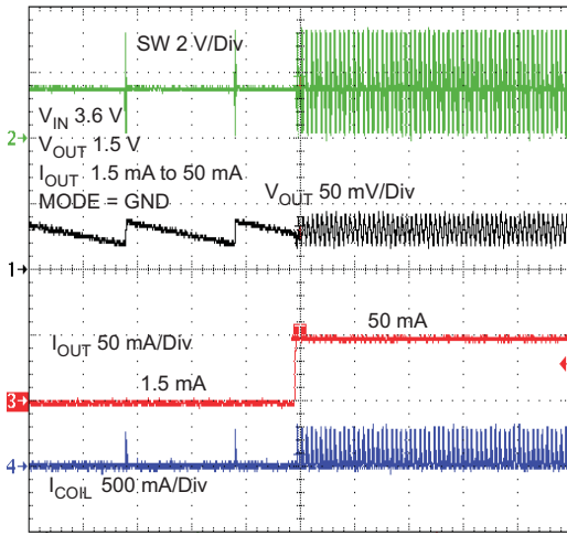
LOAD TRANSIENT (PFM Mode)
