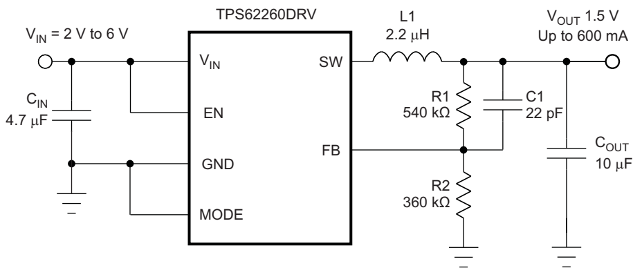
Figure 37. Adjustable 1.5-V Output
