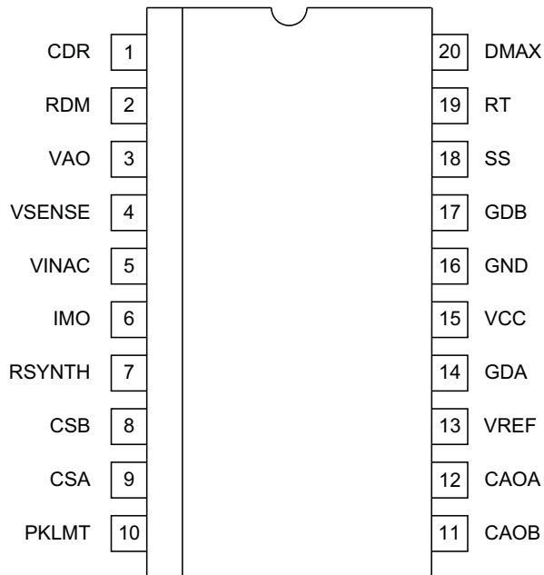
SOIC-20 Top View, DW Package
