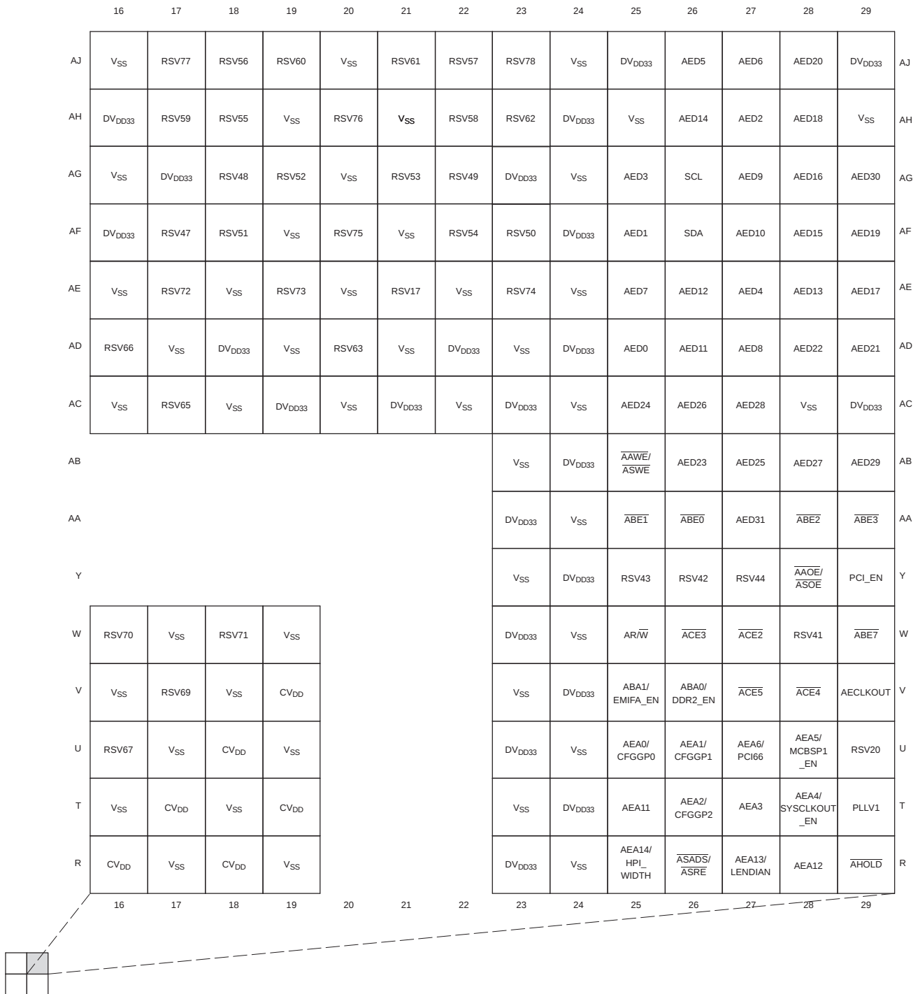
Figure 2-3. C6454 Pin Map (Bottom View) [Quadrant B]
