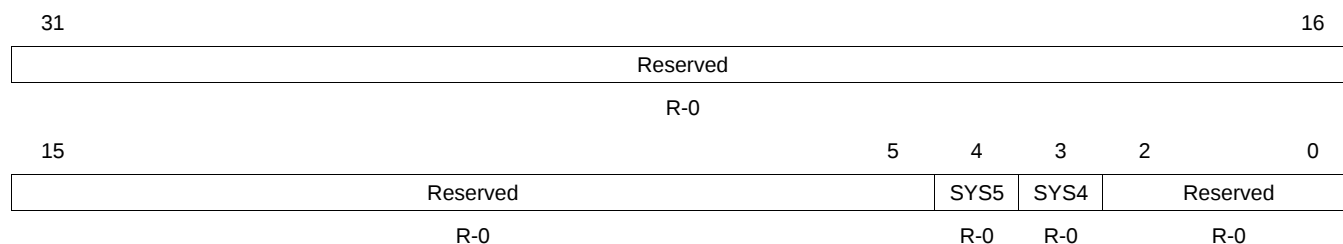
Figure 7-19. PLLDIV Divider Ratio Change Status Register (DCHANGE) [Hex Address: 029A 0144]
