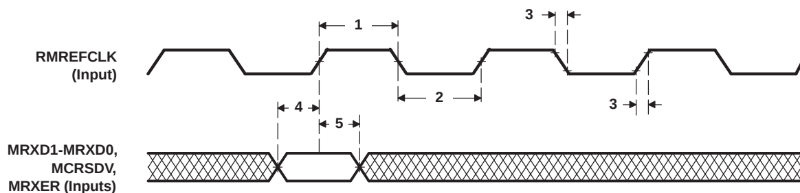
Figure 7-67. EMAC Receive Interface Timing [RMII Operation]
