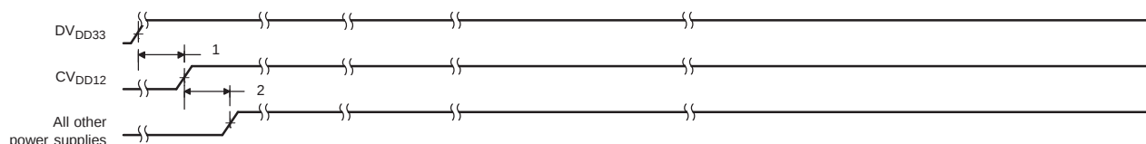
Figure 7-5. Power-Supply Sequence
