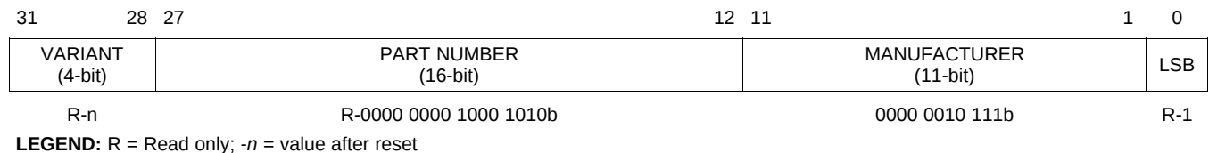
Figure 3-11. JTAG ID (JTAGID) Register - 0x02A8 0008
