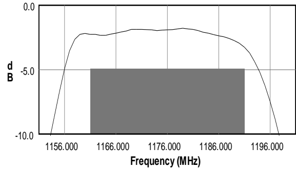
S21 Amplitude Response
