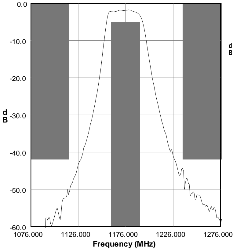
S21 Amplitude Response
